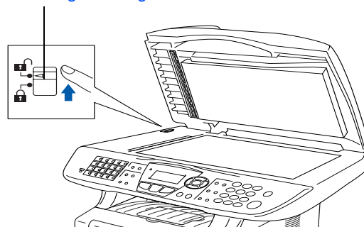
Scannervergrendelingshendel
