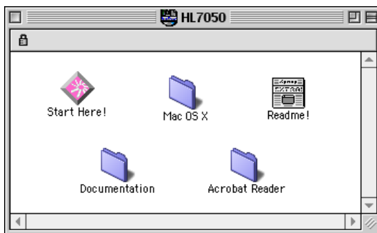
Abb. 1 Macintosh Installer
