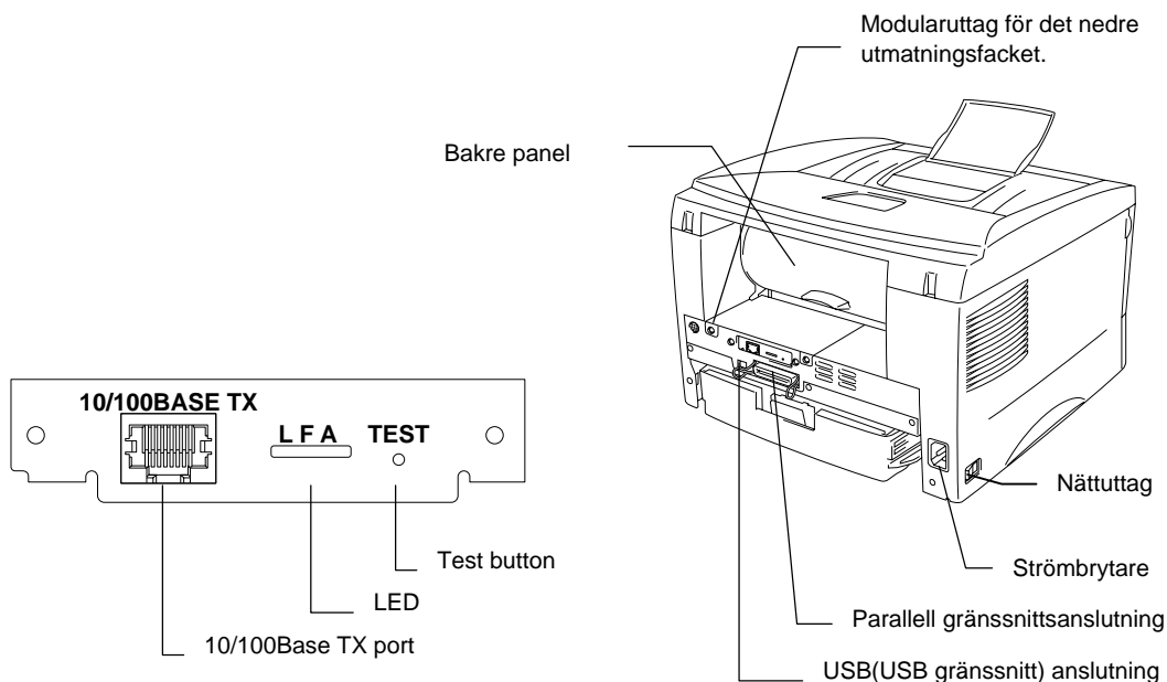
Fig. 1-3 Network Board
