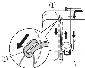
① Thread take-up lever
