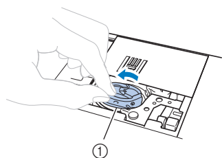
① Spulenkapsel
