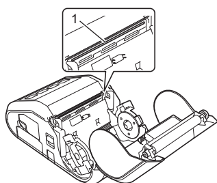
1 Printhead
